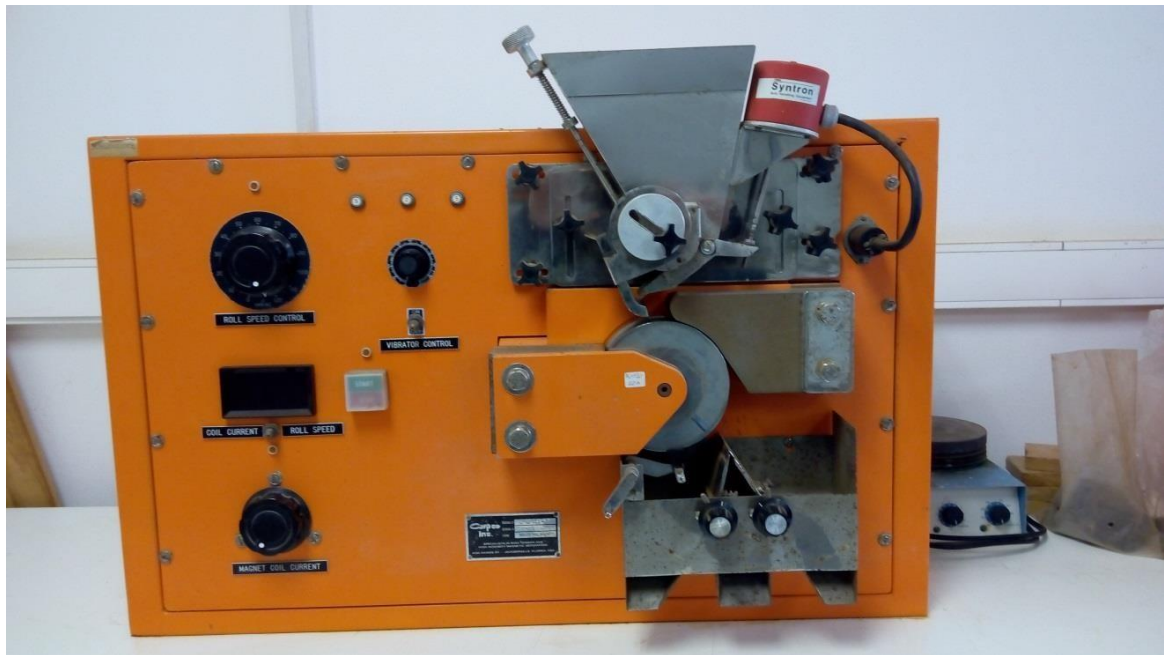
Induced magnetic roll separator (Carpco)
