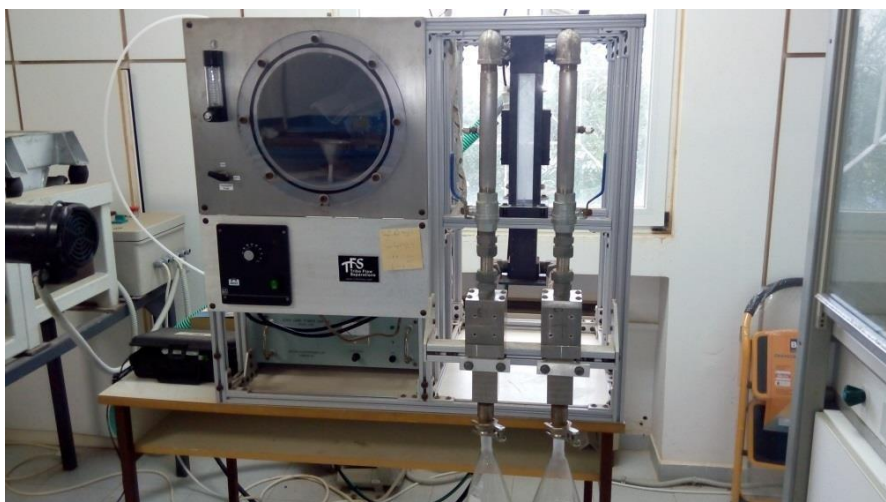
Triboelectrostatic separator (TriboFlowSeparations)
